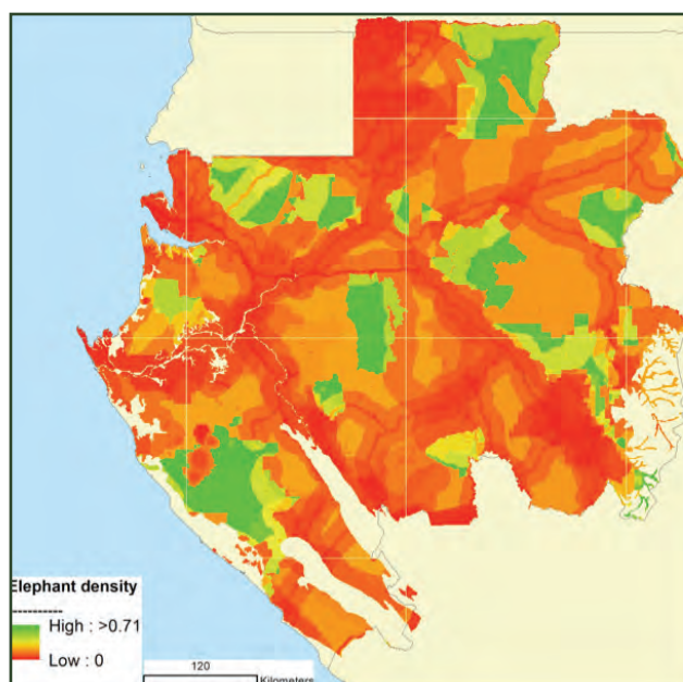
Figure 2: A model of elephant distribution in Gabon in 2011, showing density thresholds (Maisels et al. 2013). Overall density declined by 9% per year from 2002 to 2013 and likely continues to do so. Thus the high density threshold is likely lower than 0.7 in 2018.
