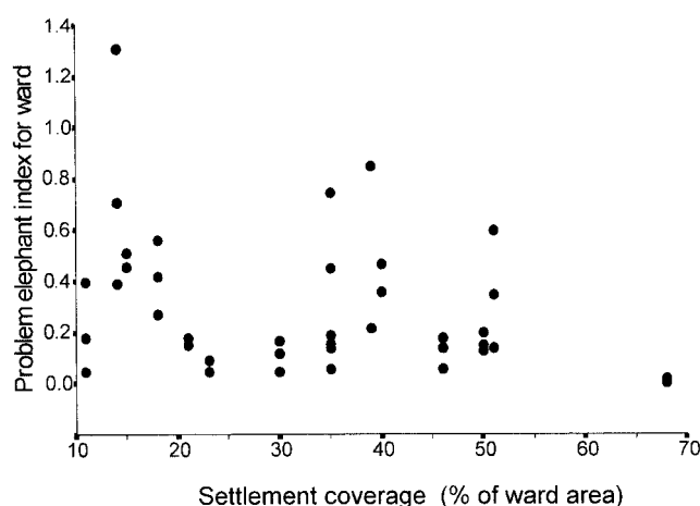
Fig. 3. The relationship between the problem elephant index (incidents \text{km}^{-2} of human settlement area per year) and settlement coverage for 15 communal land wildlife wards of the Sebungwe region, Zimbabwe.
