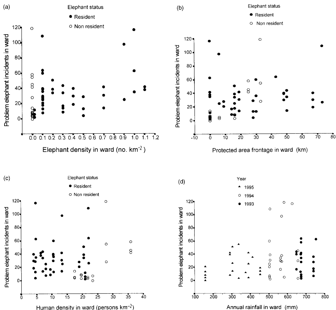
Fig. 2. The relationship between problem elephant incidents over 3 years and selected variables in 21 communal land wildlife wards in the Sebungwe region of Zimbabwe: (a) elephant density, (b) protected area frontage, (c) human density and (d) annual rainfall.
