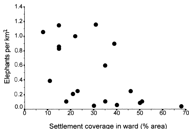
Figure 4. The relationship between the area transformed by human settlement in each Sebungwe wildlife ward and crude elephant density in the ward.
